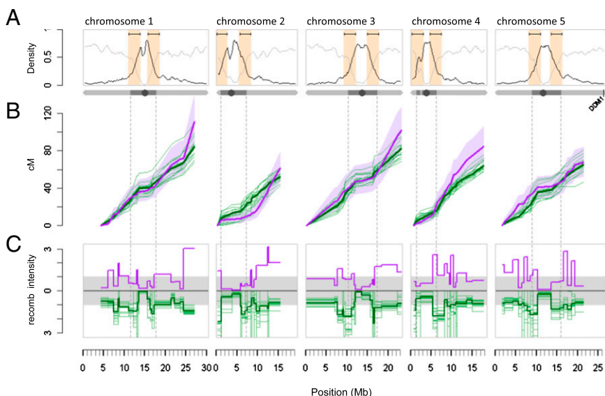
Fig. 2. Comparison of global and local recombination patterns in the epiRILs and the 17 F_2 populations (24). ( A ) Chromosome-wide gene (light gray line) and transposon (dark line) density distribution. The 3-Mb windows bracketing the intersection points between transposon- and gene-dense regions are indicated in orange. ( B ) Cumulative cM lengths of the epiRILs (thick purple line) and each of the F_2 populations (thin green lines) using the consensus map. Purple shading shows the \pm 95\% confidence interval ( C ). The thick green line denotes the average F_2 cumulative length (in cM). The dotted vertical lines define the pericentromeric regions of each chromosome. ( C ) The distribution of normalized recombination intensities (cM/Mb of a given marker interval divided by the cM/Mb chromosome average) shows suppression of recombination within pericentromeric regions and elevation at its boundaries. Color coding is as in B .
